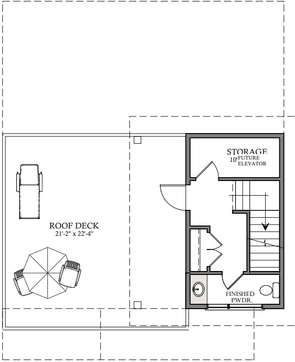
UPPER FLOOR PLAN 236 SQ. FT. - FLOOR AREA 441 SQ. FT. - DECK AREA
